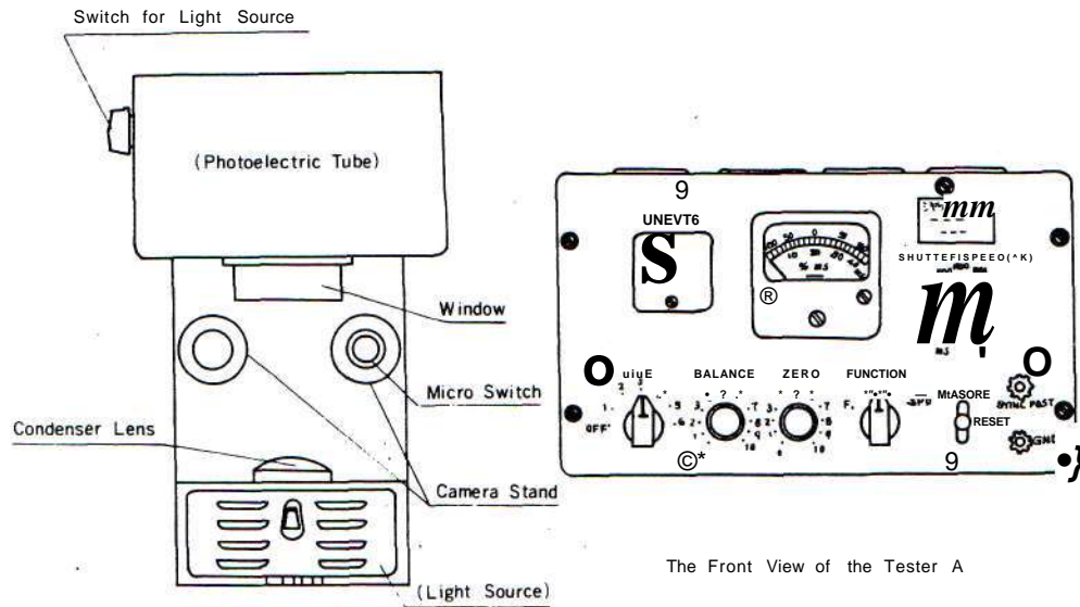
The Appearance of the lens Shutter Testers
